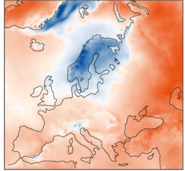
(Data: ERA5. Reference period: 1991-2020. Credit: C3S/ECMWF)
