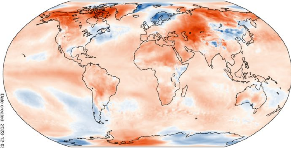
(Data: ERA5. Reference period: 1991-2020. Credit: C3S/ECMWF)
